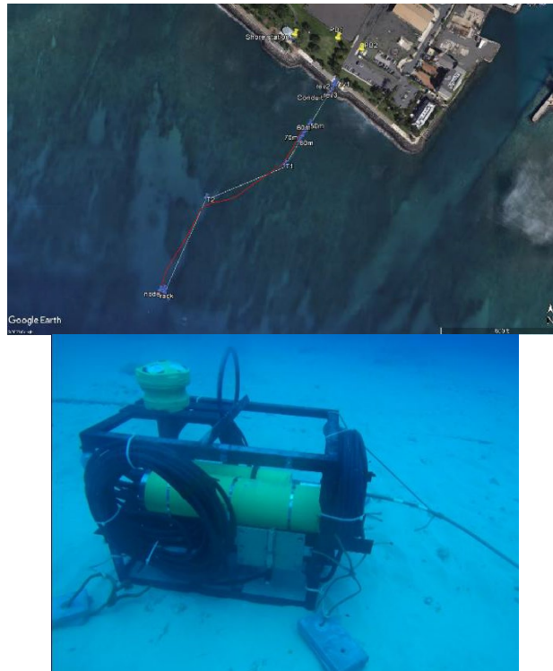
Figure 3. Kilo Nalu Observatory cable route (left) and acoustic Doppler current profiler (right).
