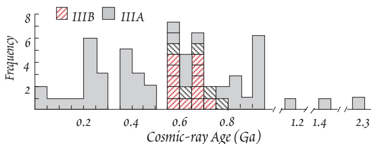
Figure 8.26. Cosmic-Ray exposure age distribution in iron meteorites. Seventeen of 18 IIIB irons fall in a cluster at 650 \pm 100 Ma (after Voshage, 1967).
