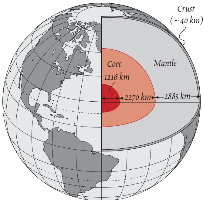
Figure 1.9. The Earth in cross-section. The outer rocky part of the planet, the mantle and crust, consists principally of silicates and is 2885 km thick. The core, divided into a liquid outer core and a solid inner core, consists of iron-nickel alloy and is 3486 km thick.
