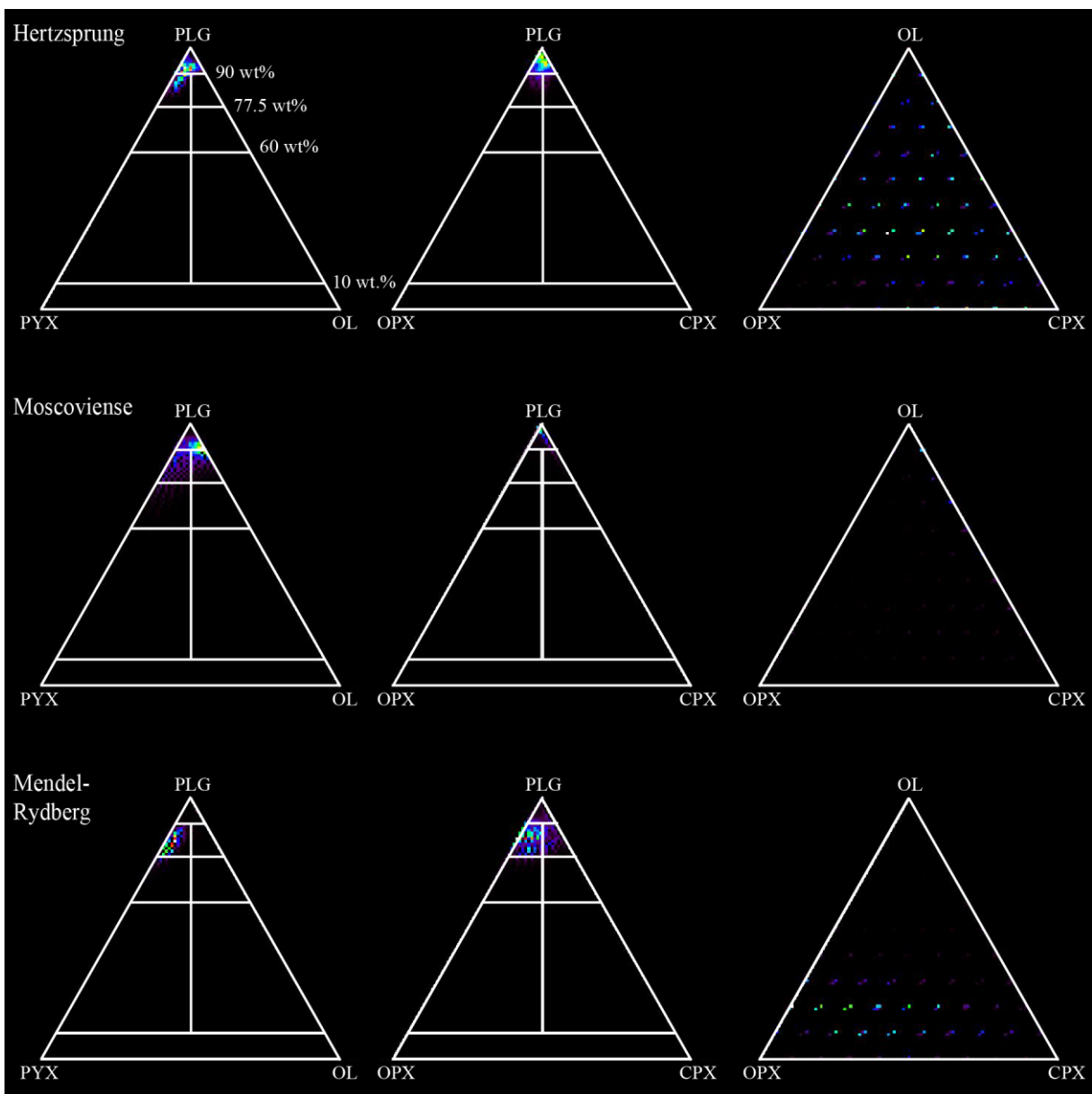
Figure C.2. Ternary diagrams showing the composition of each immature pixel (OMAT > 0.2) on the innermost ring of Hertzsprung, Moscoviense, and Mendel-Rydberg.
