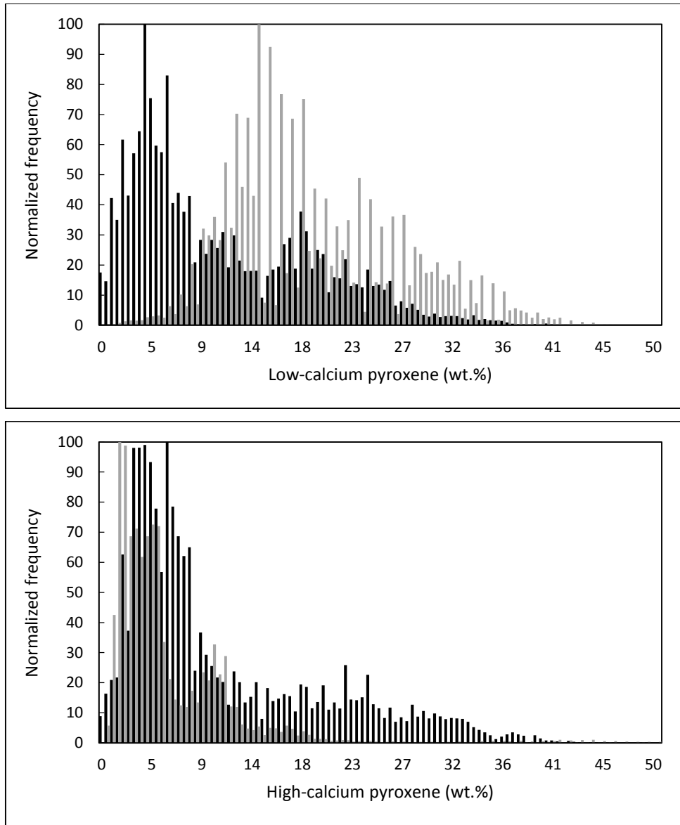
Figure 4.14. Abundance of low-calcium pyroxene and high-calcium pyroxene as derived using the Multiband Imager data within 50^\circ in latitude (black) and the Spectral Profiler poleward of 50^\circ in latitude (gray). While the Multiband Imager data suggests that low and high calcium pyroxene are present in similar abundances in the equatorial region, the Spectral Profiler data suggests that low-calcium pyroxene is much more abundance than high-calcium pyroxene in the polar region.
