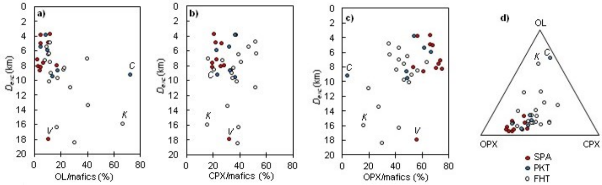
Figure 2.14. Average abundance of (a) olivine/maffics, (b) clinopyroxene/maffics, (c) orthopyroxene/maffics versus the depth of excavation ( D_{exc} ) for the 34 central peaks analyzed ( K =Keeler, C =Copernicus, V =Von Karman), and (d) ternary diagram showing the relative average abundance of each mafic mineral in these craters. The craters from South Pole Aitken basin are shown in red, from the Procellarum KREEP Terrane in blue, and from the Feldspathic Highlands Terrane in white.
