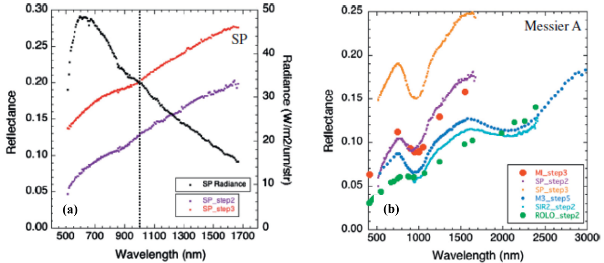
Figure 4.17. Reflectance spectra derived from various instruments and processing levels. Left: Spectra of the Apollo 6 standard site measured by the Spectral Profiler before (SP_step2) and after (SP_step3) the ground truth calibration. This figure shows the shift if the absorption band position near 900 nm before and near 1000 nm after the correction. Right: Reflectance spectra derived by various instruments at Messier A, a fresh mare region. This figure shows the difference in the position of the absorption band between the Multiband Imager data (MI_step3, near 1000 nm) and the Spectral Profiler data (SP_step2, near 900 nm). Both figures are from Ohtake et al. [2013].
