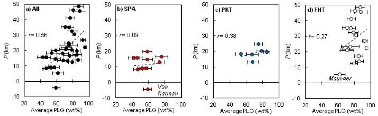
Figure 2.9. Average plagioclase (PLG) content (wt%) of the central peaks analyzed versus their proximity ( P ) to the crust mantle/boundary (km) for (a) all terranes, (b) craters within the South Pole-Aitken basin, (c) craters within the Procellarum KREEP Terrane, and (d) craters within the Feldspathic Highlands Terrane only. The variation in plagioclase content for each central peak is shown using \pm 1\sigma .
