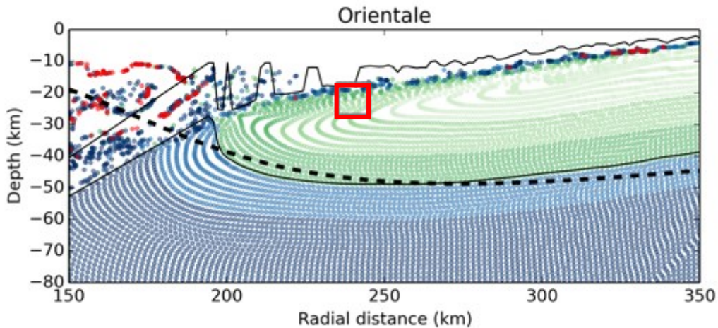
Figure 3.4. Configuration of an Orientele-like impact basin two hours after the impact, as seen by iSALE-2D. The green points represent crustal tracer particles, the blue points represent mantle tracer particles and the red points represent impactor tracer particles. The tracer particles
