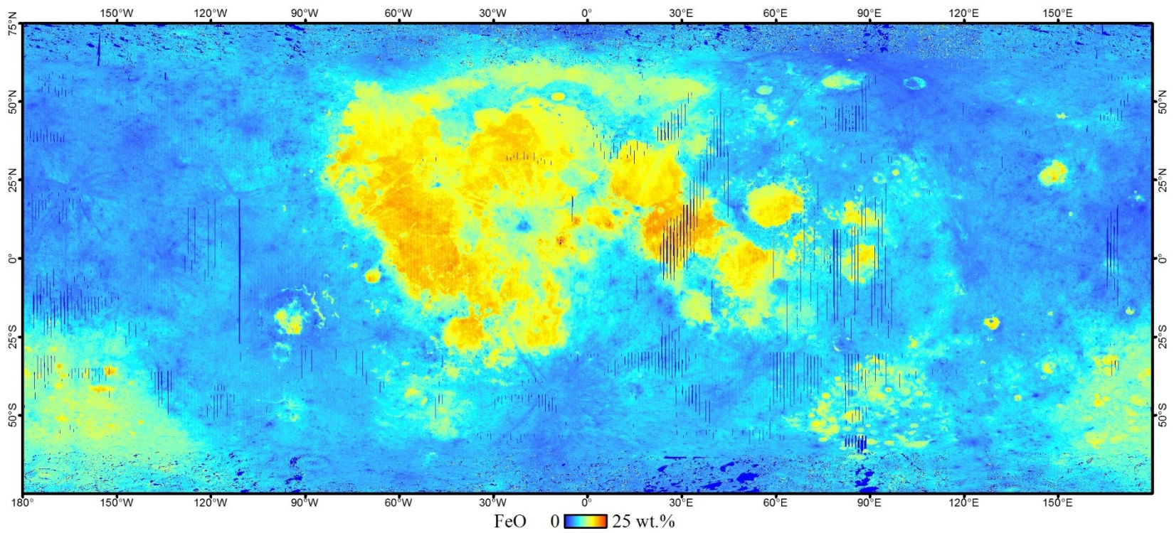
Figure B.5. Global abundance of iron as derived from the method described in Chapter Three shown here at 32 pixel per degree (~1 km per pixel).
