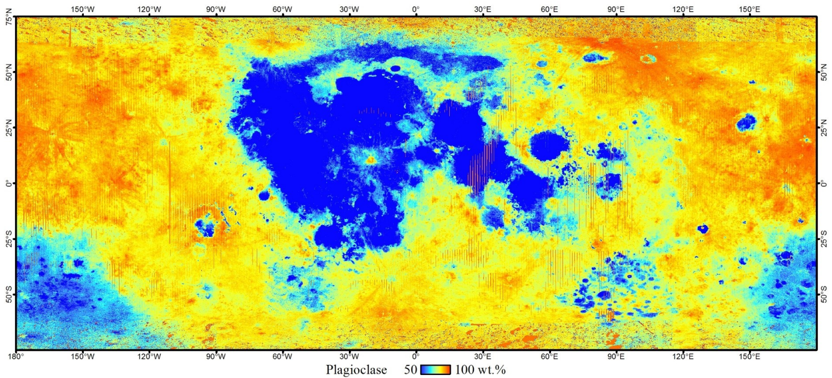
Figure B.4. Global abundance of plagioclase as derived from the method described in Chapter Three shown here at 32 pixel per degree (~1 km per pixel).
