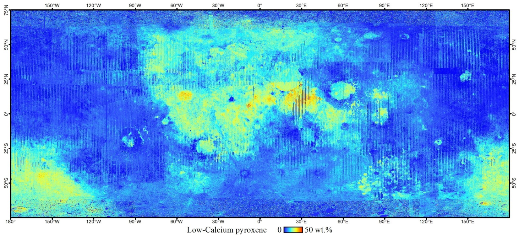
Figure B.2. Global abundance of low-calcium pyroxene as derived from the method described in Chapter Three shown here at 32 pixel per degree (~1 km per pixel).
