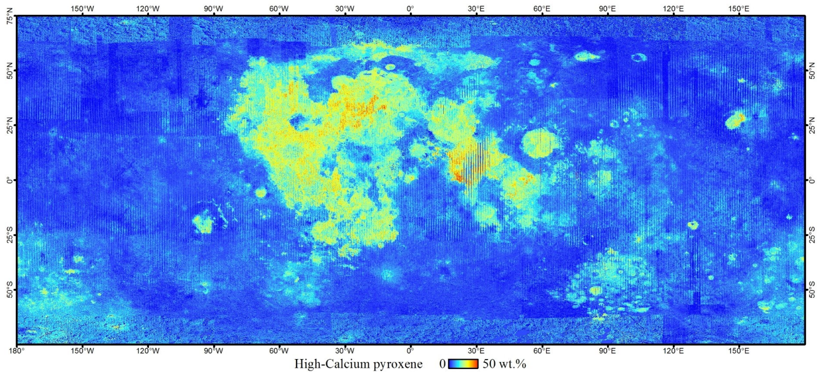
Figure B.3. Global abundance of high-calcium as derived from the method described in Chapter Three shown here at 32 pixel per degree (~1 km per pixel).
