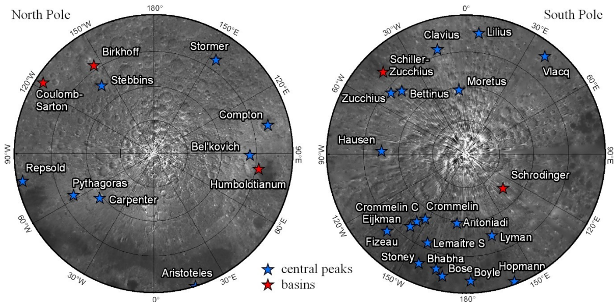
Figure 4.1. Location of the 27 central peaks (blue stars) and 5 basin rings (red stars) analyzed in this study poleward of 50^\circ latitude. The background is the reflectance measured by the Spectral Profiler at 955.4 nm, scaled from 0 to 0.4 black to white, using orbits 2000-2700 in the north polar region, and orbits 4124-4998 in the south polar region.
