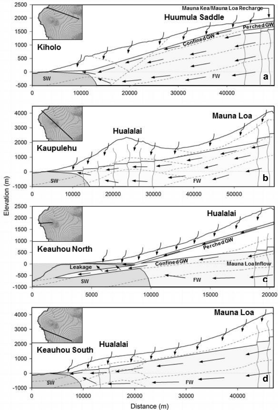
Figure 3.7(a-d). Conceptual hydrologic cross sections of Kīholo (a), Kaūpūlehu (b), Keauhou North (c), and Keauhou South (d) transects. Solid black lines define land surface, water table, and freshwater (FW)-seawater (SW) interface. Dashed gray lines are approximations of subsurface structure, while solid gray lines indicate dikes. Freshwater extent is light gray while seawater extent is dark gray. Straight arrows indicate groundwater flow direction in the saturated zone while curved arrows indicate recharge.
