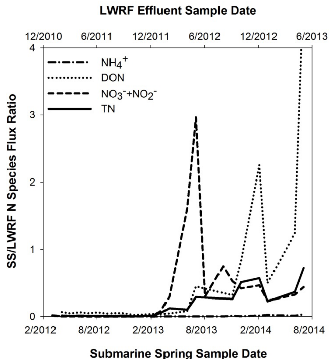
Figure 2.11: Ratios obtained by dividing submarine spring N species flux by LWRF N species flux determined 14 months prior to the indicated date to account for travel time. The ratios of all N species fluxes except for \text{NH}_4^+ increase dramatically after February 2013.
