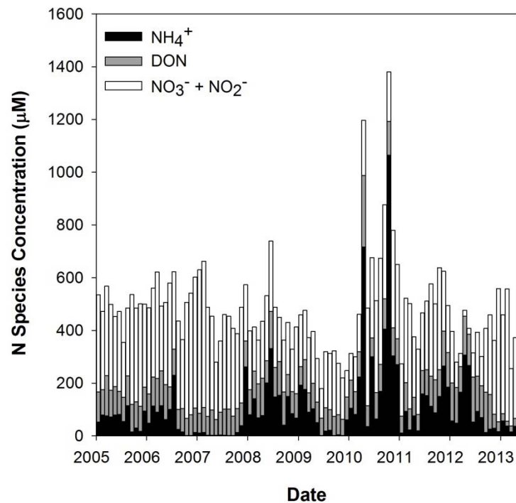
Figure 2.2: LWRF effluent monthly average N species concentrations from January 2005 to May 2013. Note that the anomalously high TN values are generally associated with high \text{NH}_4^+ concentrations.
