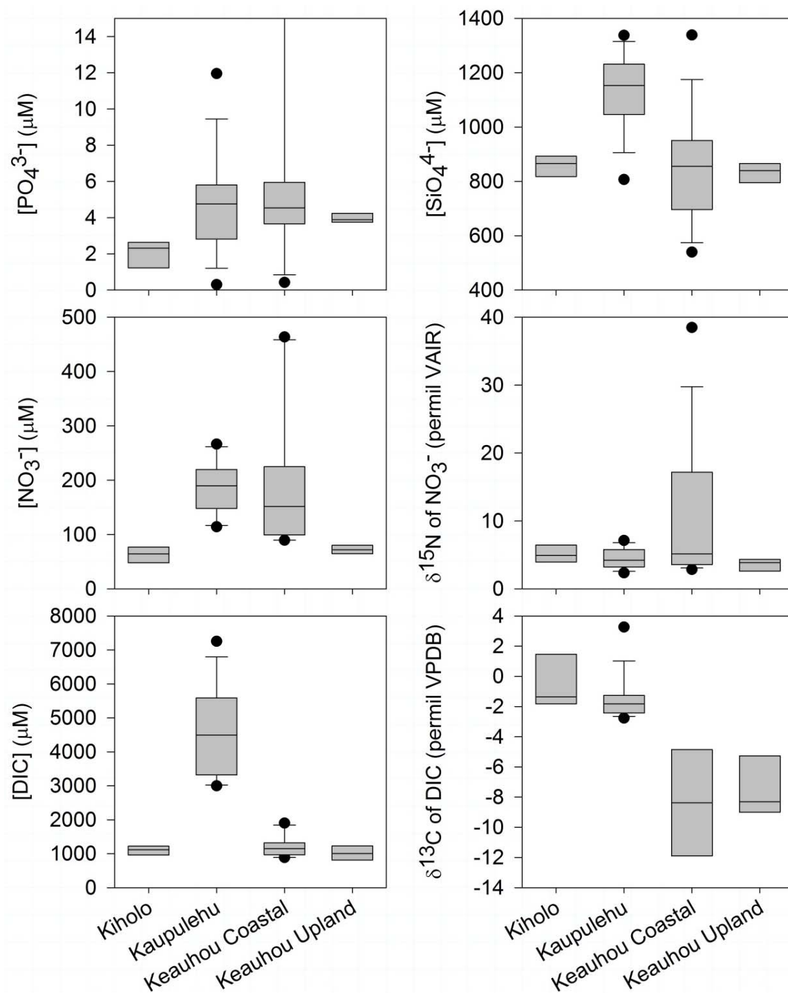
Figure 4.3. Box plots of salinity and indirect recharge unmixed groundwater nutrient, DIC, and stable isotope parameters grouped by region. The boundaries of the gray box represent the 25 th and 75 th percentiles, while the center line represents the median. For groups with n > 8 , whiskers indicate the 10 th and 90 th percentiles and outliers are represented as points. For the Keauhou Coastal \text{PO}_4^{3-} plot, Expansion Well 2 ( [\text{PO}_4^{3-}] = 127.19 \mu\text{M} ) is not pictured for clarity.
