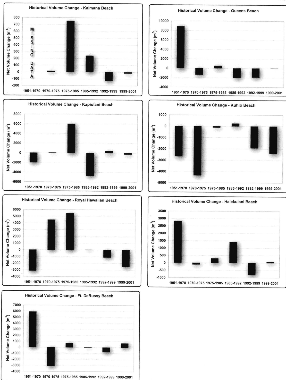
Figure 9. Volume change for historical time intervals by littoral cell.
