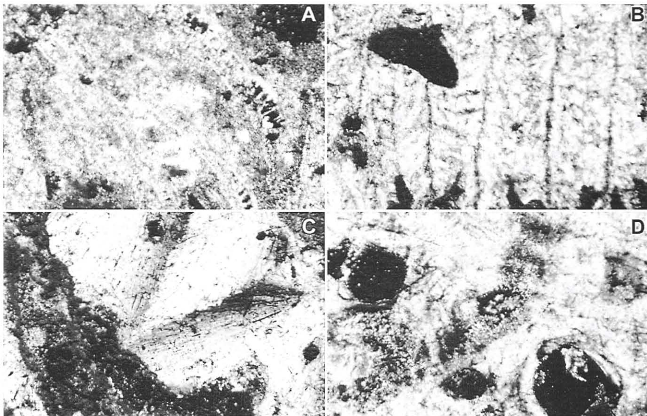
FIG. 4.—Lithofacies. A) Coral-algal bindstone from Hale O Lono (21 m depth) with encrusting coral and heavy laminar micritic cement displaying knobby texture. This lithofacies occurs at both HOL and Hikauhi. B) Massive coral framestone from Hikauhi (10.7 m depth). This lithofacies occurs only at Hikauhi. C) Mixed skeletal rudstone from Hale O Lono (8.5 m depth) showing brachiopod fragment and knobby micritic cement (lower left). This lithofacies occurs only at HOL. D) Branching coral framestone-bafflestone from Hale O Lono (17.7 m depth) showing bored, branching Porites compressa with aragonitic cement. This lithofacies occurs only at HOL.
