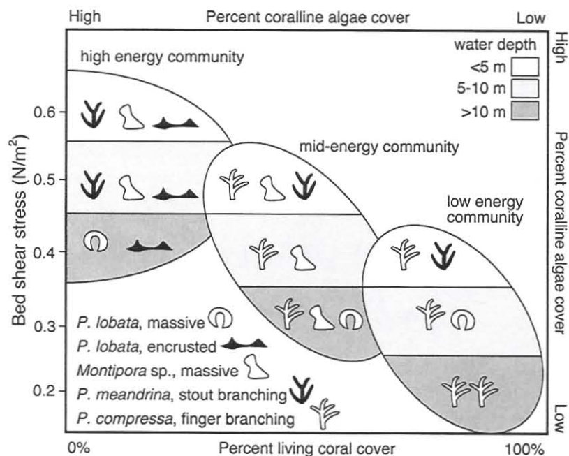
FIG. 8.—Model of modern coral assemblage zonation. This model relates bed shear stress (WINBSS) with percent living coral cover, dominant coral species, and coral morphologies. The low-energy community is dominated by Porites compressa , especially at depths > 5 m, and is found along the central portions of the south shore of Molokai. To the west, bed shear stress increases and the ecosystem shifts to a mid-energy community, as at Hikaui, dominated by Porites compressa and Montipora sp. At the westernmost site, Hale O Lono, near the western end of the island where bed shear stresses increase sharply, the high-energy community is dominated by Porites lobata , Pocillopora meandrina , and Montipora sp.
