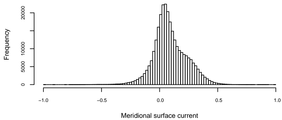
Figure 5: Frequency distributions of the sea surface temperature (SST), zonal surface current (ZSC) and meridional surface current (MSC).
