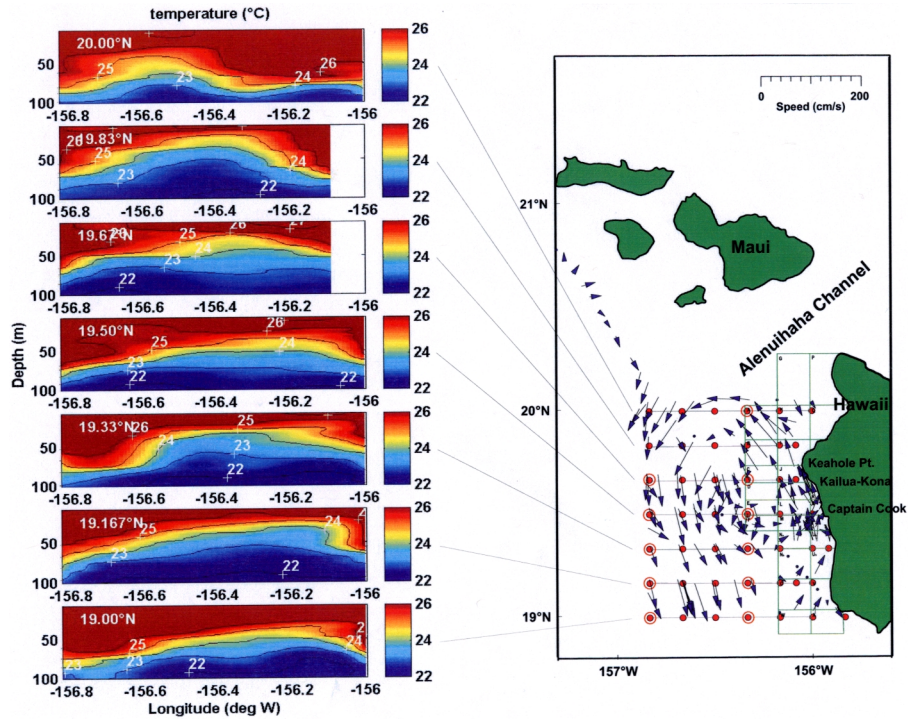
Fig. 1. (a) Temperature sections with respect to depth for seven zonal sampling lines aboard the Townsend Cromwell (TC), 26 July–5 August 1995. (b) Oceanographic station sampling grid (filled red dots); WOCE drifter deployment positions (second red circles) and schematic vector representation of estimated current velocities and direction along the TC cruise track. Current vectors have length scales to reflect relative velocities current speeds and direction averaged over the upper 21–100 m. Green gridlines correspond to statistical areas for the HIBT.
