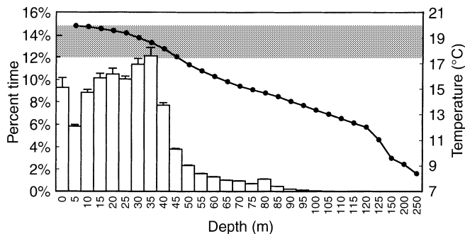
Fig. 7 Thunnus albacares . Percent occupancy of temperature intervals as a function of depth (data points joined by line indicate mean water temperatures at each depth; shaded area encompasses >90% of total time and highlights preference of species for water temperatures >17.5 °C; depth intervals = 0 to 4.999 m; 5 to 9.999 m; 10 to 14.999 m, etc.)
