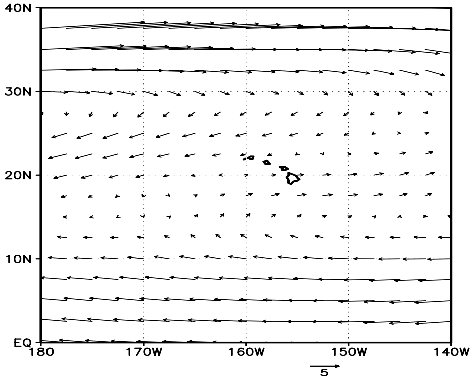
Figure 6.19. Climatological (1966-2003) mean TLMW ( \text{m s}^{-1} ) in June.
