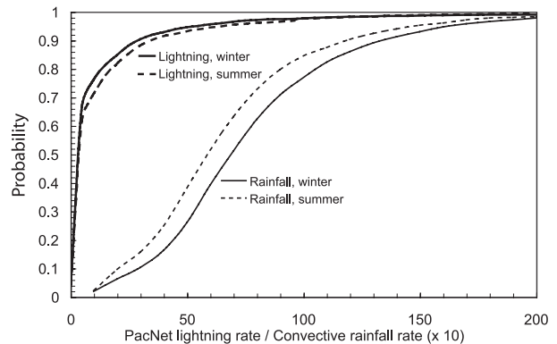
FIG. 3. Cumulative PDF for PacNet lightning rate [flashes \times (10^4 \text{ km}^2 \text{ h})^{-1} ] and PR convective rainfall rate ( \text{mm h}^{-1} \times 10 ). The x axis is suppressed with \sim 99\% of the highest rates shown.
