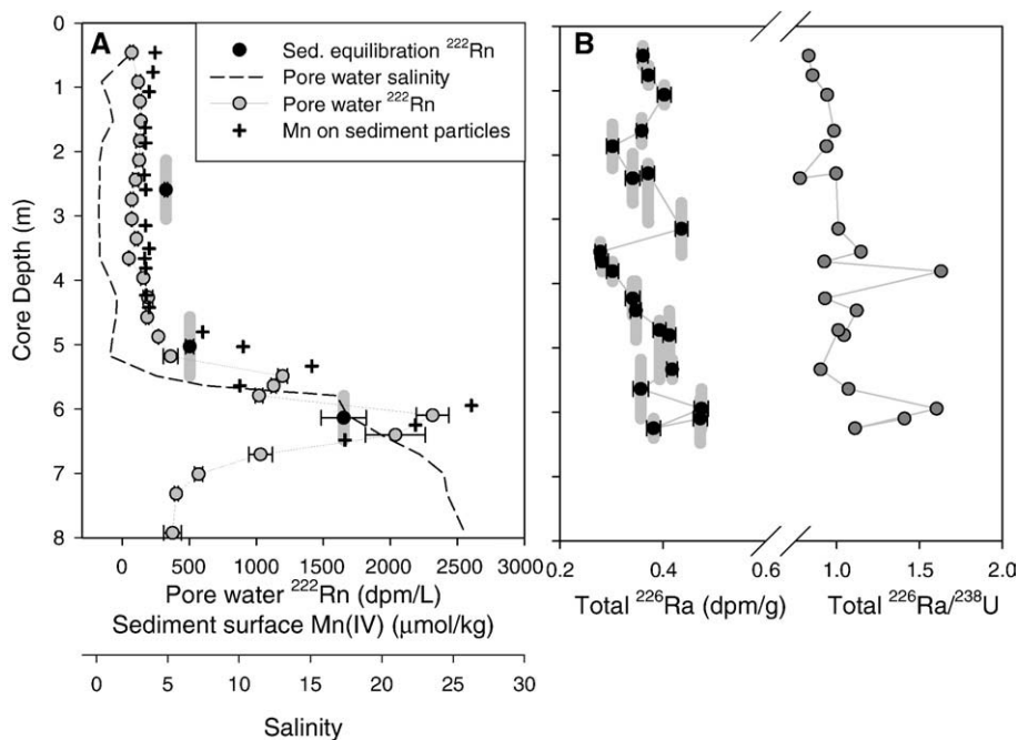
Fig. 3. A. Pore water salinity (dashed line) and ^{222}\text{Rn} (grey circles, dpm L -1 ), sediment bound Mn (crosses, \mu\text{mol kg}^{-1} ) and sediment equilibrium ^{222}\text{Rn} (black circles, dpm L -1 ) measured in June 2006 plotted against depth (m). The vertical uncertainty bars on the sediment equilibrium ^{222}\text{Rn} values represent the depth range of sediments mixed together for each sample. B. Total bulk sediment ^{226}\text{Ra} (dpm g -1 ) and ^{226}\text{Ra}/^{238}\text{U} ratios measured by gamma-spectrometry. The vertical uncertainty bars on the bulk ^{226}\text{Ra} values represent the depth range of sediments mixed together for each sample.
