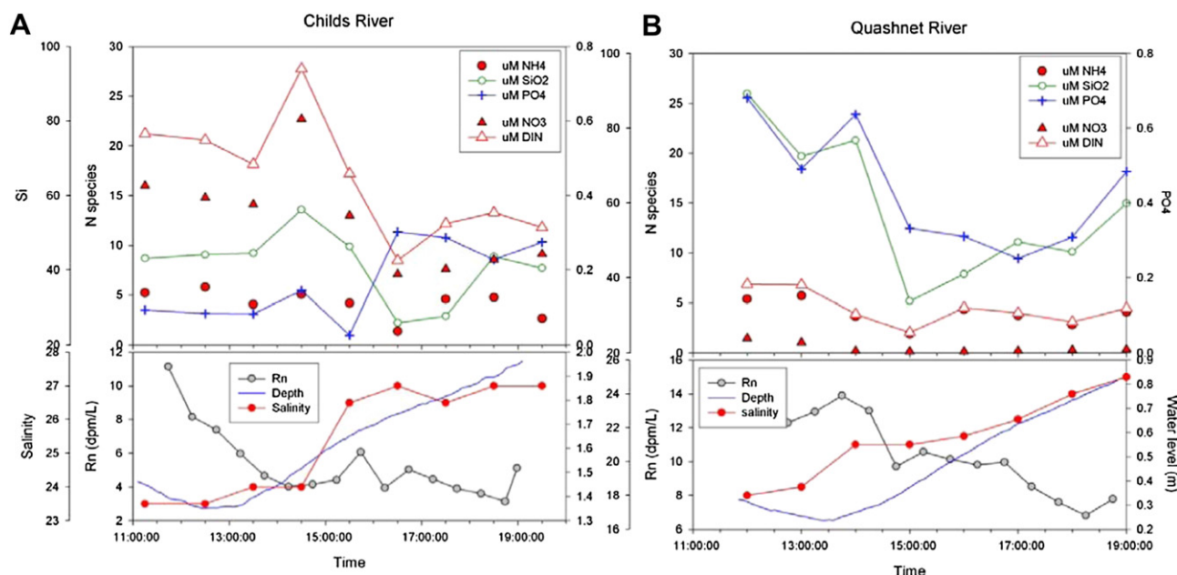
Fig. 9. Time series measurements of radon, salinity and nutrients for a period of a change of low tide to high tide in (A) Childs River and (B) Quashnet River on Dec 5, 2007. Water level, nitrate + nitrite, ammonium, phosphate, silicate, DIN, radon and salinity parameters are indicated over an 8-h period.
