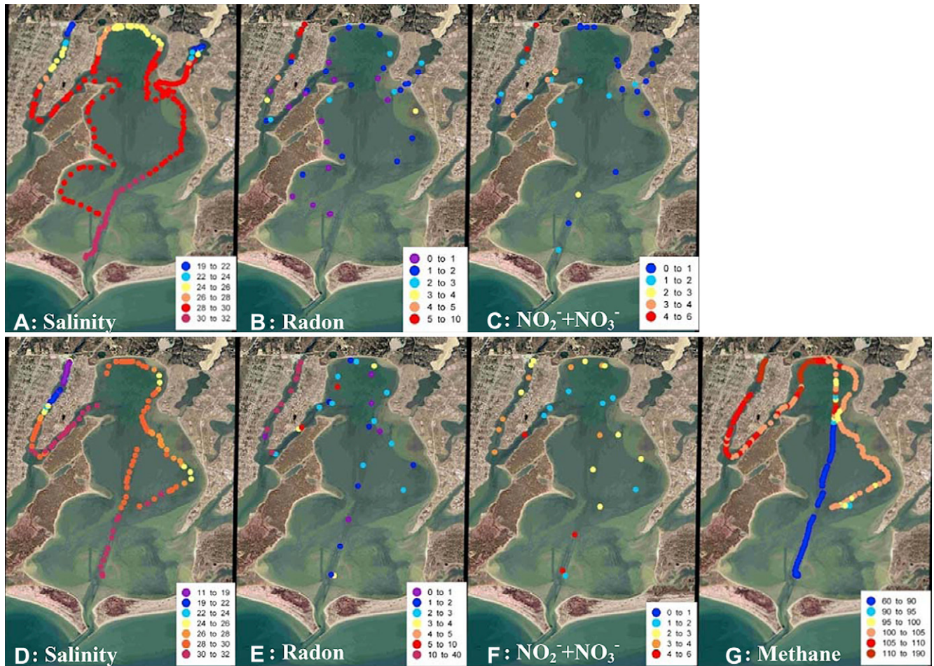
Fig. 6. Summer (A–C) and winter (D–G) coastal surface water survey results from Waquoit Bay showing salinity (A, D); radon in \text{dpm L}^{-1} (B, E); nitrate + nitrite in \mu\text{M} (C, F); and methane in relative units (G, winter only). Warm colors are high and cold colors are low values as indicated on each legend. Due to low water levels we were not able to survey Quashnet River in such detail as the other parts of the bay.
