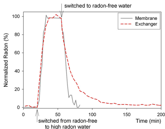
Fig. 2. Response time of Liquicel and the air–water gas exchanger to changes in radon activities in water. First, radon-free water was passing through both systems, after 20 min the water intake was switched to high radon activity water, and after 55 min the water intake was switched back to radon-free water. Ten minutes after switching from high radon to radon-free water intake 10% of the radon remains in the Liquicel system. The same 10% level is reached in the air–water gas exchanger after 45 min.
