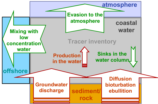
Fig. 4. Sources and removal processes that influence radon/methane inventory in the coastal water. The input terms are indicated by brown arrows and loss terms by green arrows, and the tracer fluxes represent the interactions between sediments, coastal water, atmosphere, and offshore water.
