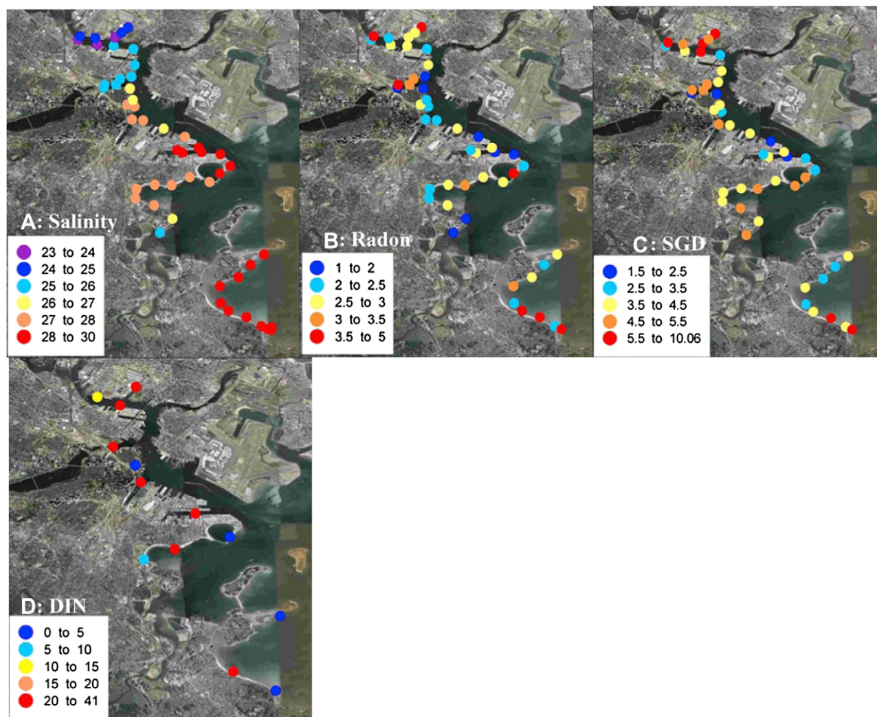
Fig. 7. Coastal surface water survey results from Boston Harbor showing (A) salinity; (B) radon in \text{dpm L}^{-1} ; (C) submarine groundwater discharge in \text{m}^3 \text{m}^{-1} \text{d}^{-1} ; and (D) ammonia + nitrate + nitrite in \mu\text{M} .
