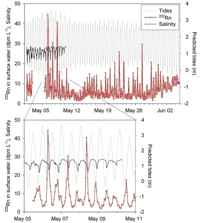
Fig. 5. Long-term monitoring of radon, water level, and salinity in Savin Hill Cove in Boston Harbor. The inset is zoomed in on a selected time period that shows a clear negative correlation between salinity/tides and radon. At high tide the water is diluted by low radon high salinity offshore water, at low tides fresh/brackish SGD lowers salinity and brings in new radon that is then mixed away with the next flood tide.
