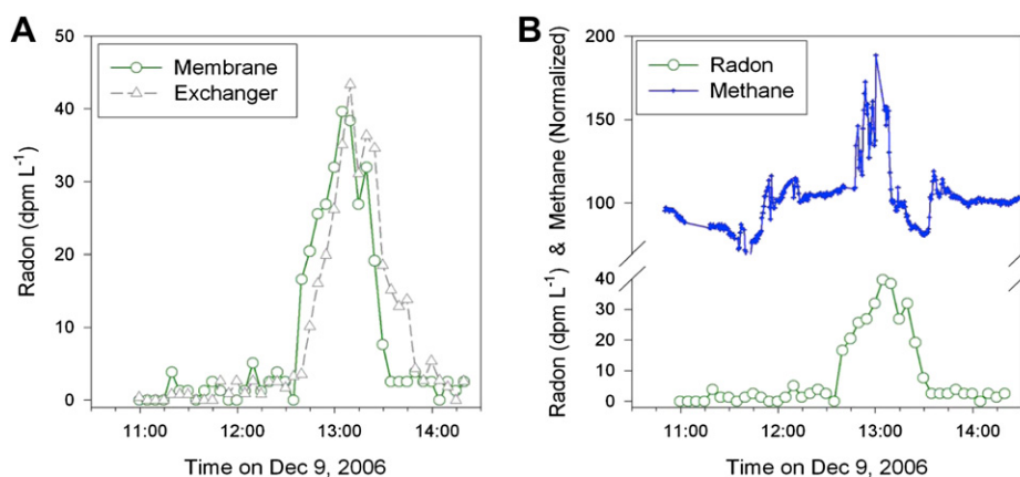
Fig. 3. (A) Radon measured during a survey in Waquoit Bay, MA with two different radon mapping systems, one system used a classic air–water exchanger and the other the newly tested membrane. Both systems were run in 5 min integrated intervals and their water intakes were positioned to sample the same water parcel. For easier comparison, radon values are plotted against time instead of geographical reference points. (B) Simultaneous radon and methane survey in Waquoit Bay, MA. Radon is smoothed out spatially because it has been measured in a continuous 5-min integrated measurement intervals, whereas methane values were recorded every 30 s. Values are plotted against time of sample collection.
