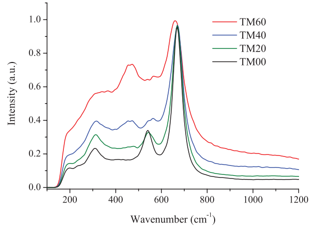
FIGURE 4. The average Raman spectra for each TM sample before background correction. (Color online.)
