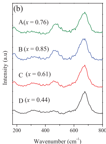
FIGURE 7. (a) A reflected light image of the region within a titanomagnetite grain in melatroctolite sample analyzed by electron probe microanalyzer (EPMA) and Raman spectroscopy: ilm = ilmenite; tmt = titanomagnetite; ple = pleonaste. Circles are spots analyzed by EPMA and crosses are spots analyzed by Raman. (b) Raman spectra of the four different spots shown in a. The x values were found using Equations 1 and 2. For A–C, Equation 2 was not applicable because the peak T_{2g}(2) was not discernible. (Color online.)
