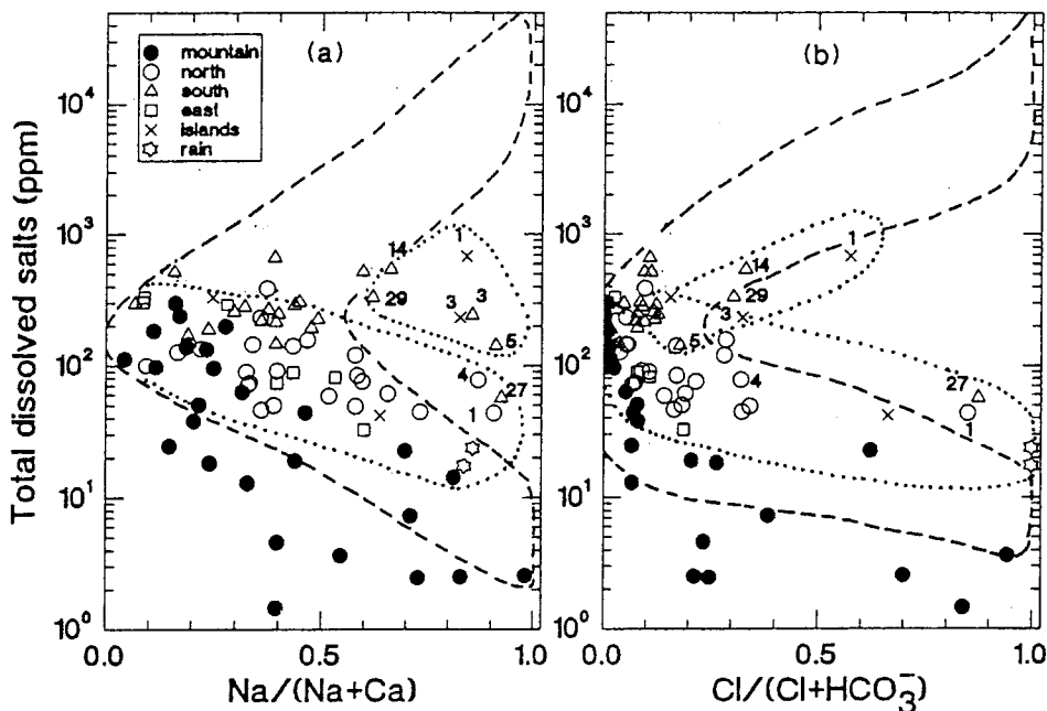
Fig. 13. Plots of the total dissolved salts versus the weight ratios of Na/(Na + Ca) and Cl/(Cl + HCO 3 ) for the world-wide surface waters (fields enclosed by dashed lines, given by Gibbs, 1970), and for water samples from Taiwan's lakes and reservoirs. The dotted lines enclose normal coastal samples and some unusual samples discussed in the text. Numerals are specific sample numbers given in Table 1.
