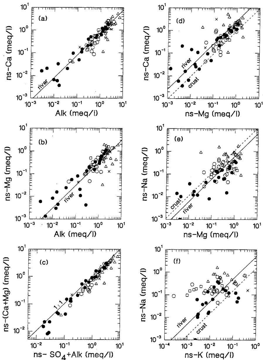
Fig. 9. Correlation plots of various pairs of chemicals. The preface "ns" represents the non-seasalt component. The solid diagonal line in each diagram represents the ratio of a given chemical pair for the world mean river water, and the dotted lines the ratios for the average upper crust of Taiwan.
