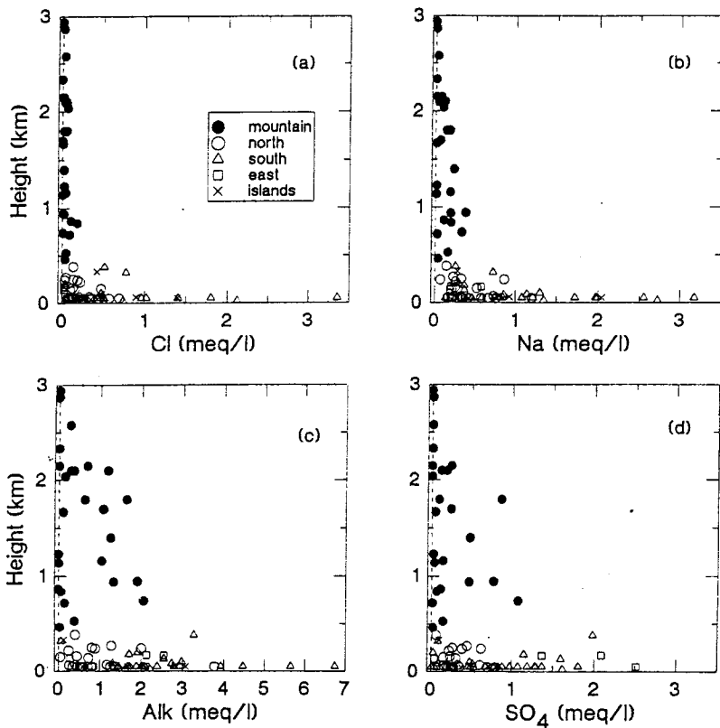
Fig. 7. Plots of altitude versus (a) Cl, (b) Na, (c) Alkalinity, and (d) SO 4 concentrations in lake and reservoir waters.
