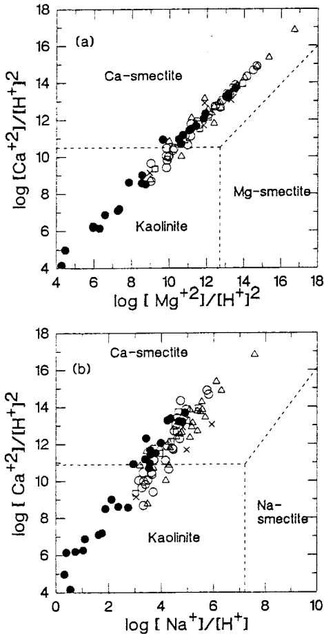
Fig. 12. Activity- activity diagrams and stability fields of Ca-, Mg- and Na-smectite and kaolinite.
