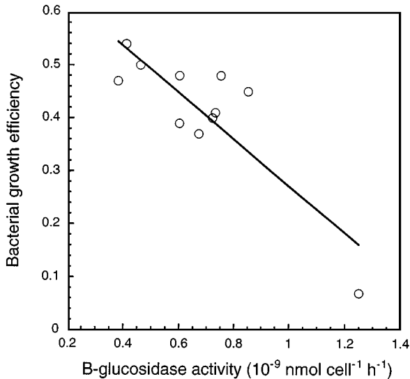
Figure 6 Relationship between BGE and \beta -glucosidase activity in lake bacterioplankton. Data from Middelboe & Søndergaard (91).
