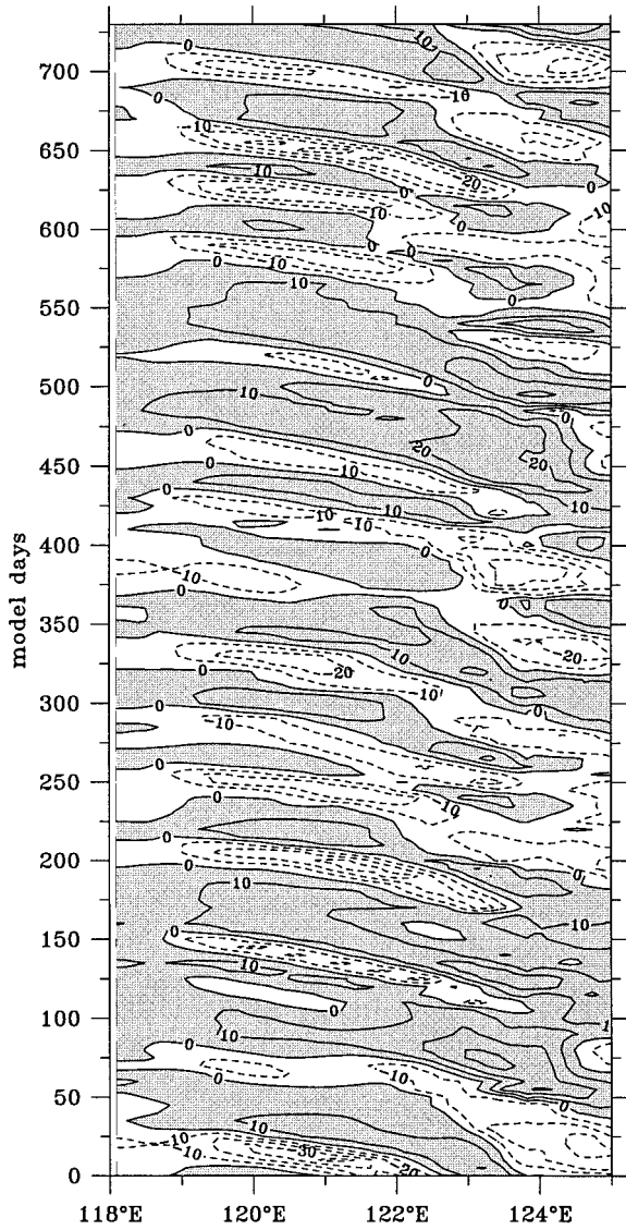
FIG. 12. Time-longitude diagram of the upper-layer thickness anomalies from the base model run along the center latitude ( 4^{\circ}\text{N} ) of the Celebes Sea. Unit in meters.
