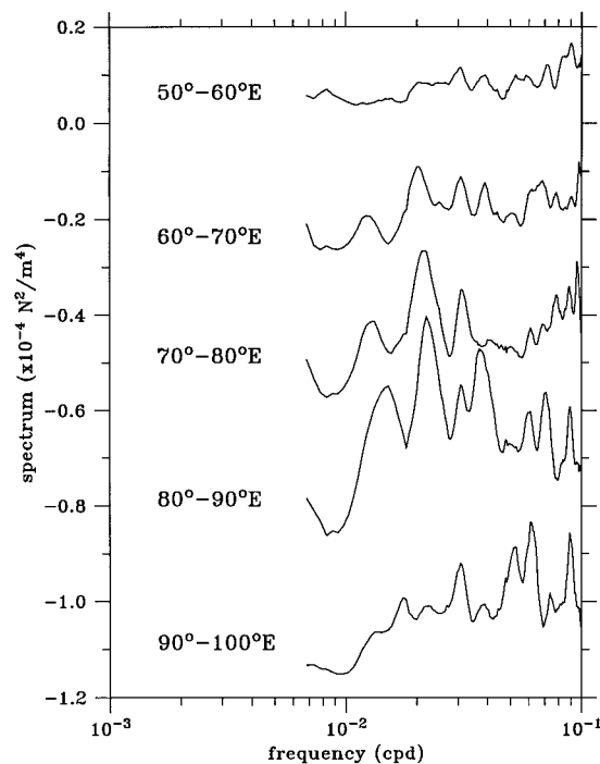
FIG. 18. Power spectra of the zonal wind stress in the intraseasonal frequency band (10–150 days) along the equator from 50° to 100°E. The power spectra are based on the daily 1000-mbar ECMWF wind data and are averaged in five 10°-wide segments. The power spectra for each segment are shown with an offset of 0.3 \times 10^{-4} \text{ N}^2 \text{ m}^{-4} .
