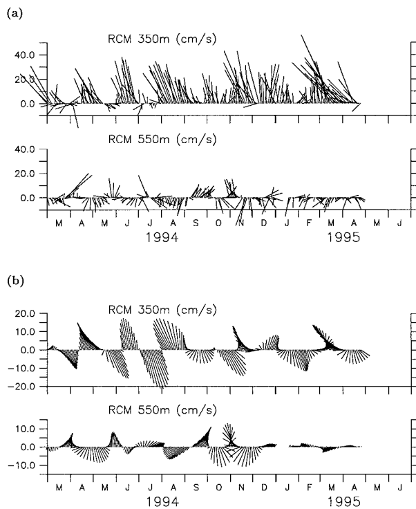
FIG. 2. Time series of velocity vectors from moored current meters deployed at the entrance of the Celebes Sea ( 4.0^{\circ}\text{N} , 127.5^{\circ}\text{E} ). (a) Observed velocity vectors at the 350-m and 550-m depths. (b) Velocity vectors after 30-to-120 day bandpass filtering. Adapted from Watanabe et al. (1997).
