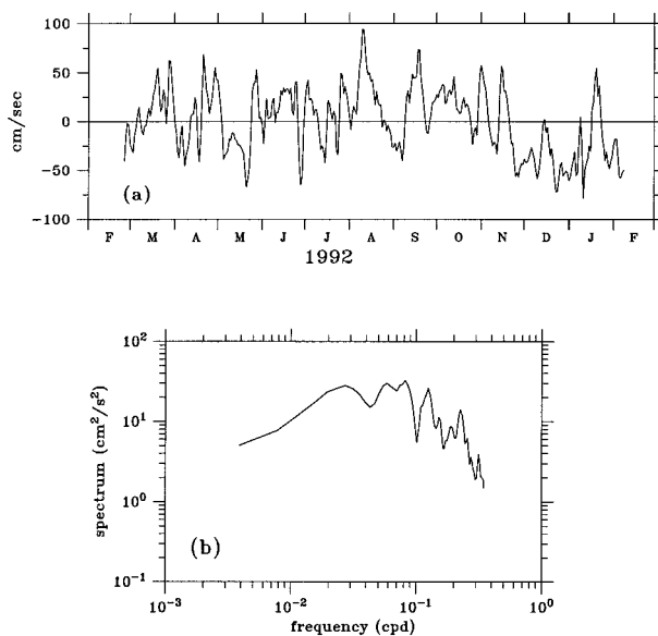
FIG. 3. (a) Time series of the first EOF mode for the alongchannel flow at 11.3°S, 122.9°E in the Timor Passage (from Fig. 9a of Molcard et al. 1996). (b) Power spectra of the time series shown in variance preserving format.
