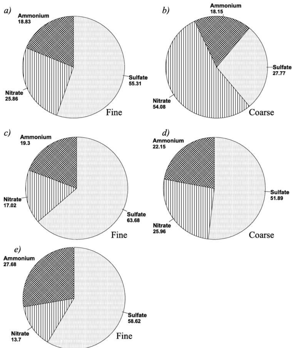
Figure 8. Mass percentages of submicron and supermicron secondary ions when the trajectory C (a, b) passed nearby Shanghai, (c, d) arrived at P-3 flight 9 at 6:55 GMT, and (e) PILS observation at 6:55 GMT.
