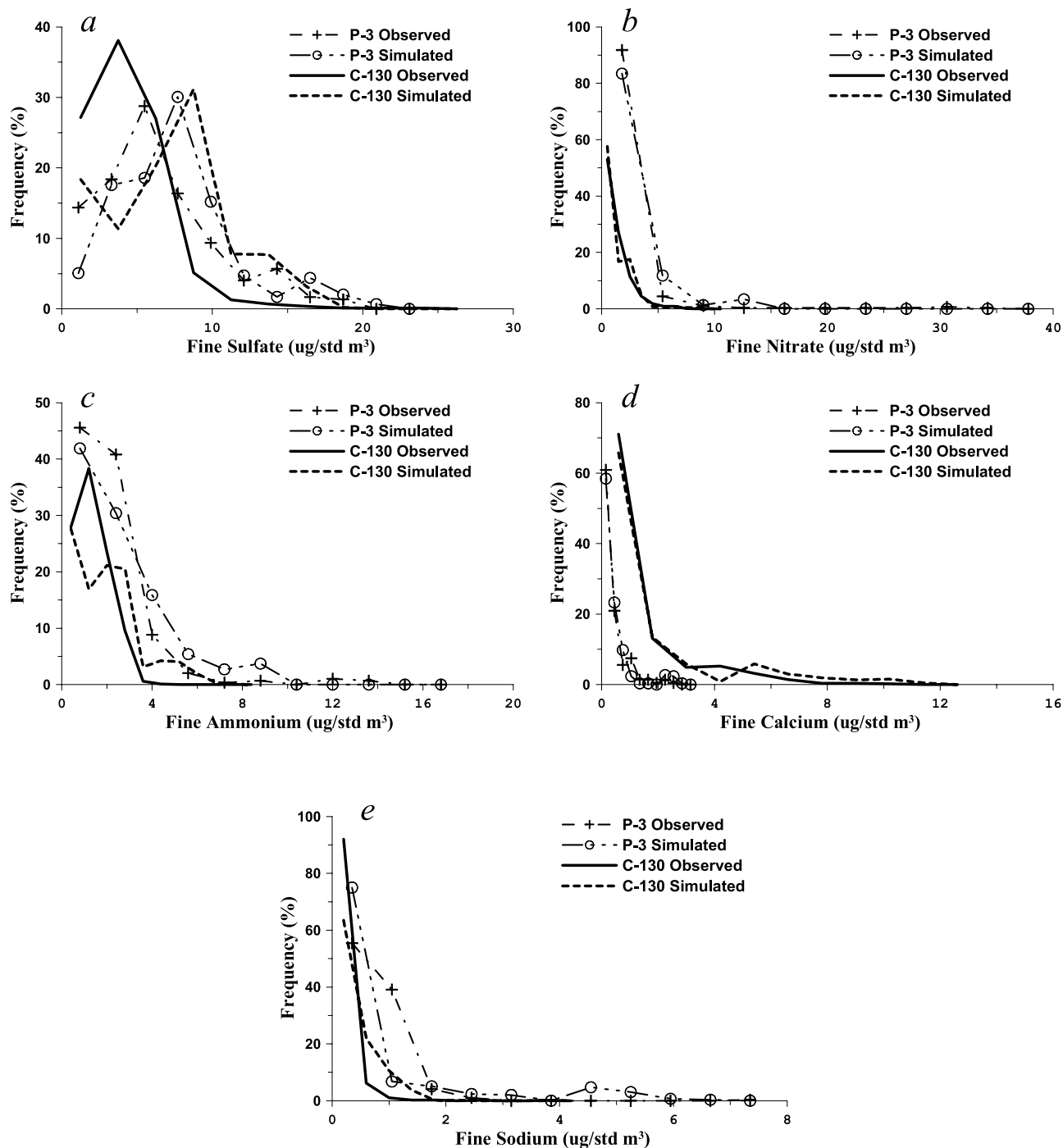
Figure 16. Simulated and observed frequency distributions (%) of fine aerosol concentrations below 1 km for all TRACE-P P-3 and ACE-Asia C-130 flights: (a) sulfate, (b) nitrate, (c) ammonium, (d) calcium, and (e) sodium.
