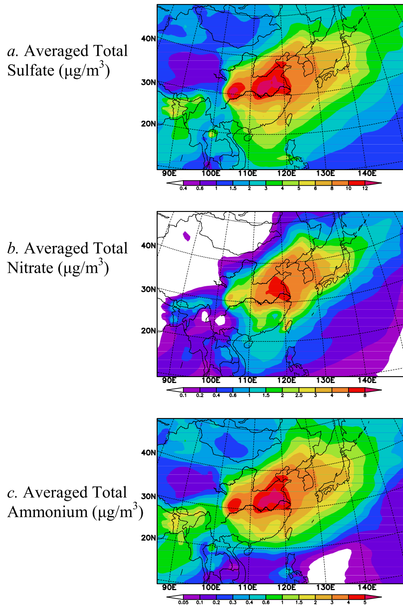
Figure 1. Simulated mean sulfate, nitrate, and ammonium concentrations at 400 m level for March and April.
