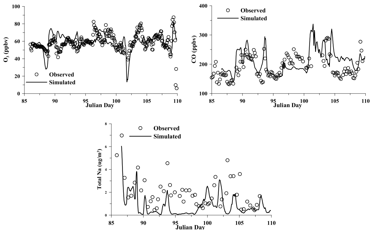
Figure 14. Simulated and observed O_3 , CO, and total sodium concentration along the cruise path of the R/V Ronald Brown . The aerosol ion was measured with two-stage multijet cascade impactor [Quinn et al. , 2000].
