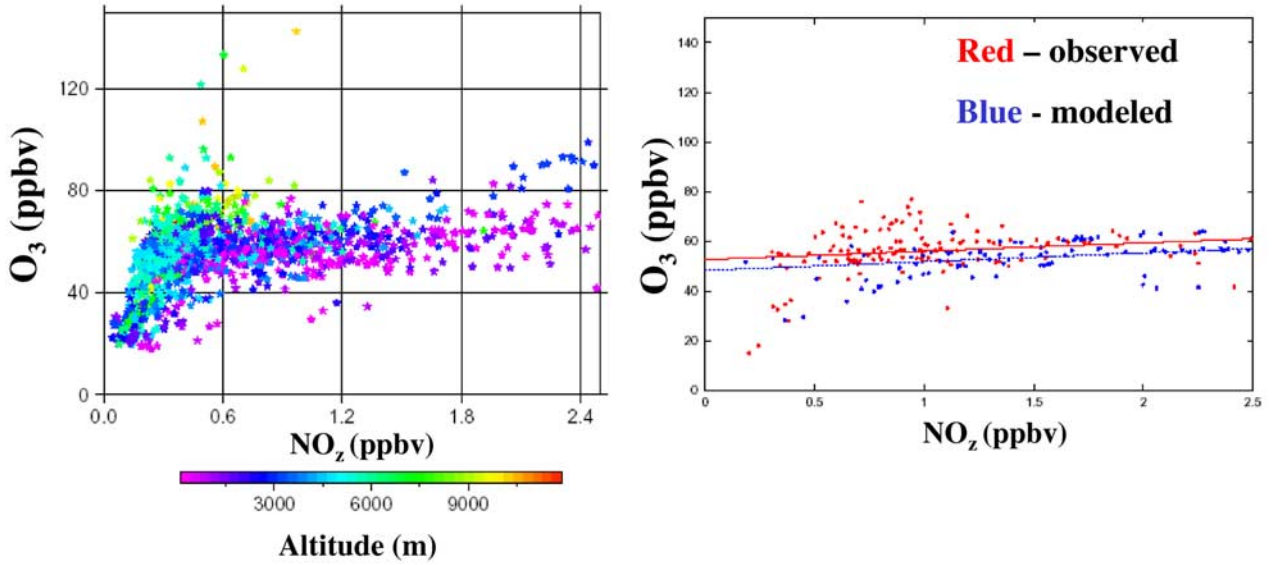
Figure 19. Observed relationship between O_3 and NO_z based on DC8 and P3 data (5-min merged) colored in altitude of the observation (a); ozone production efficiencies for points identified by back trajectory analysis to have passed over Central China at altitudes below 2 km (b). The red dots represent the observation points identified by the back-trajectory analysis; the blue dots represent the model values for these same points.
