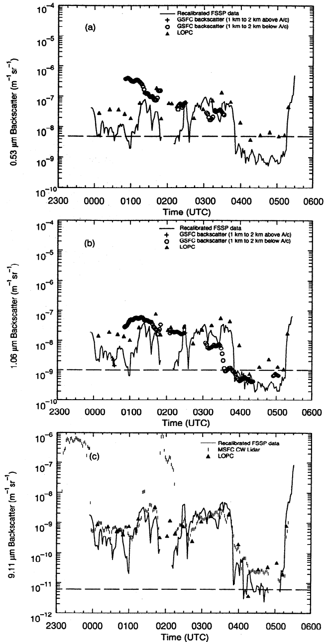
Figure 4. Temporal variation of measured and modeled aerosol backscatter coefficient ( \beta ) during flight 14 for wavelengths (a) 0.53 \mu\text{m} , (b) 1.06 \mu\text{m} , (c) 9.11 \mu\text{m} , (d) 9.25 \mu\text{m} , and (e) 10.59 \mu\text{m} . Dashed line in each panel represents the lidar detection threshold.
