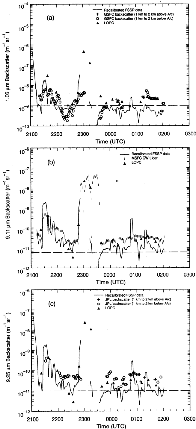
Figure 3. Temporal variation of measured and modeled aerosol backscatter coefficient ( \beta ) during flight 6 for wavelengths (a) 1.06 \mu\text{m} , (b) 9.11 \mu\text{m} , and (c) 9.25 \mu\text{m} . Dashed line in each panel represents the lidar detection threshold.
