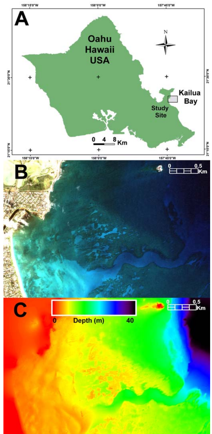
Figure 2. Study site location and data. (A) Map of Oahu, Hawaii. Study site within Kailua Bay is outlined. (B) Initial QuickBird image for study site, displayed as an RGB image. (C) Shoals LIDAR data interpolated to a depth image and displayed in rainbow hues varying from red at 0 m to black at 40 m.
