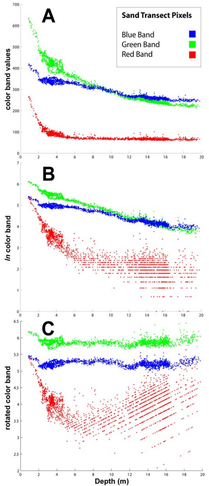
Figure 3. Plots of sand transect pixels for each stage of the process. (A) Initial data. Sand transect pixels for blue, green, and red bands are plotted with depth values on the x-axis and color band DN values on the y-axis. (B) \ln -transformed data. Sand transect pixels are plotted with depth values on the x-axis and \ln -transformed DN values on the y-axis. (C) Rotated data. Sand transect pixels are plotted with depth values on the x-axis and rotated color band values on the y-axis.
