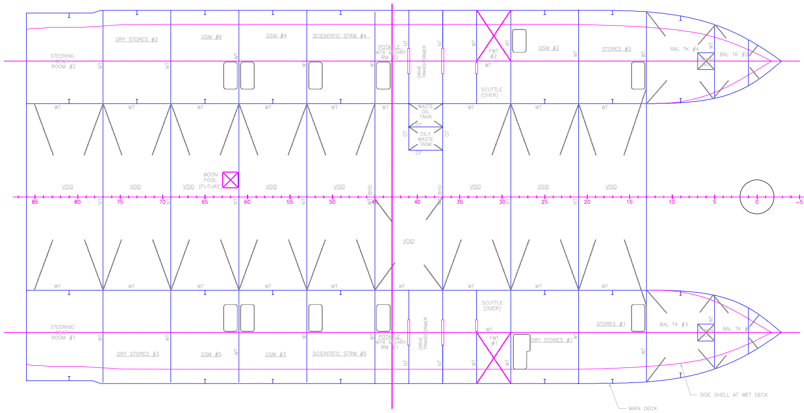
PLAN VIEW - WET DECK
