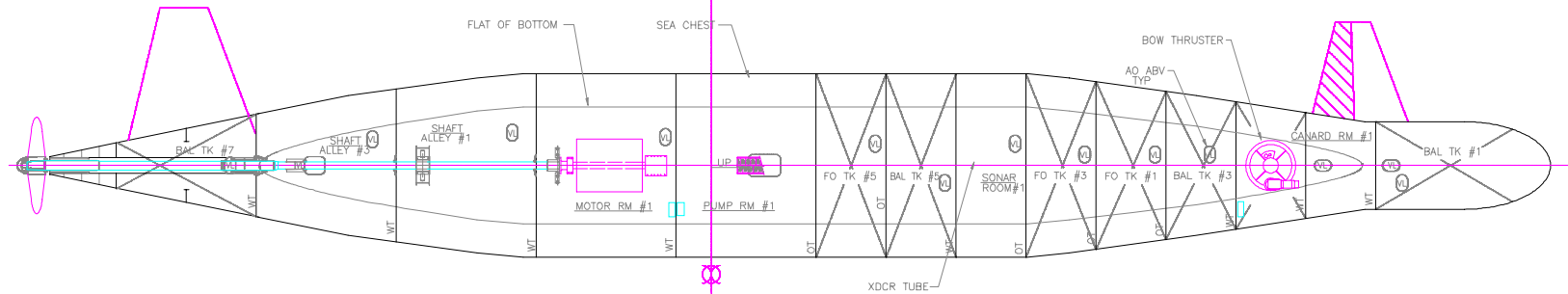
PLAN VIEW - 3RD PLATFORM
