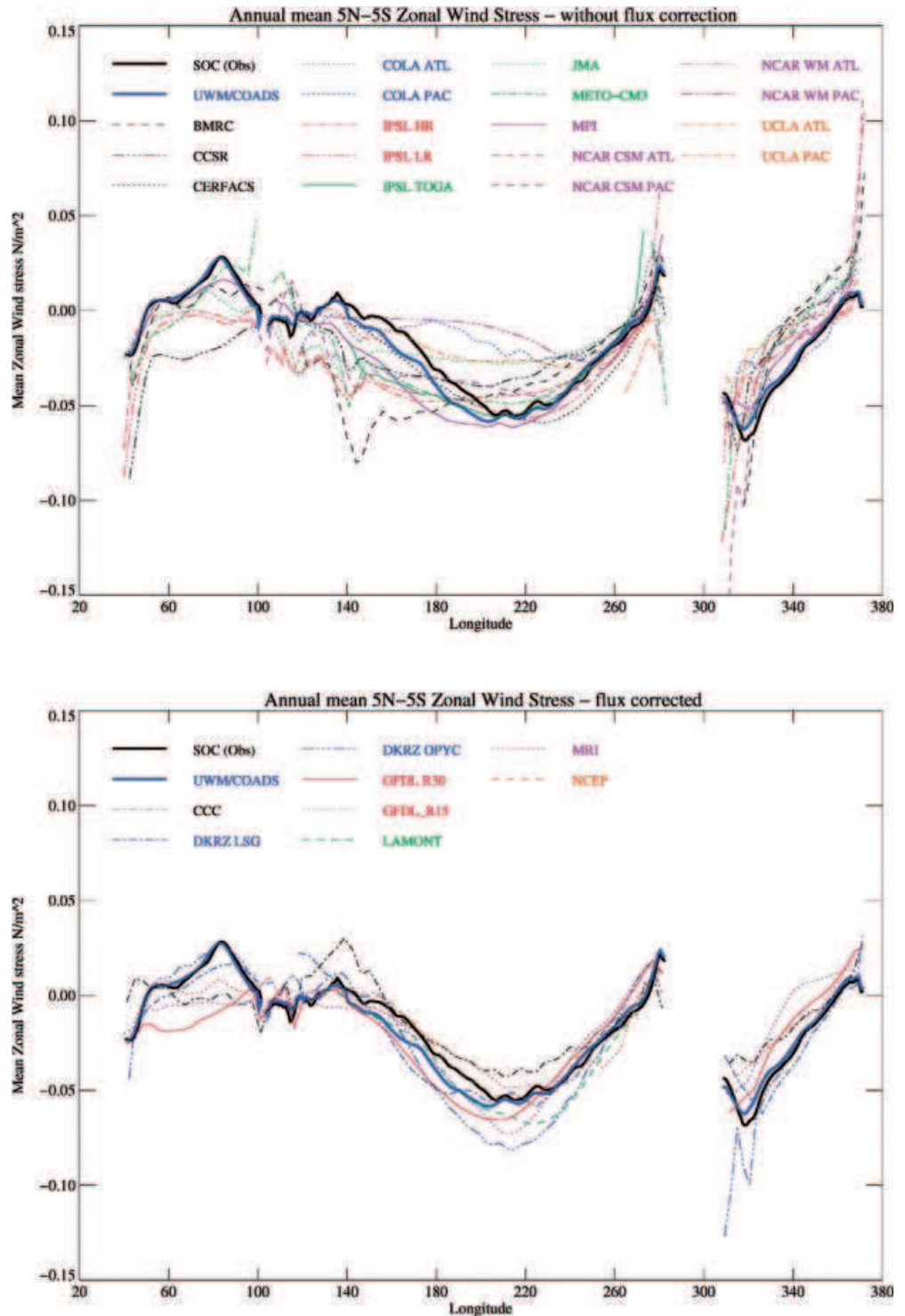
Fig. 2 Annual mean zonal wind stress zonal section in the equatorial strip 5°N-5°S, as observed and for (top) ‘no-adj’ CGCMs, (bottom) ‘adj’ CGCMs
