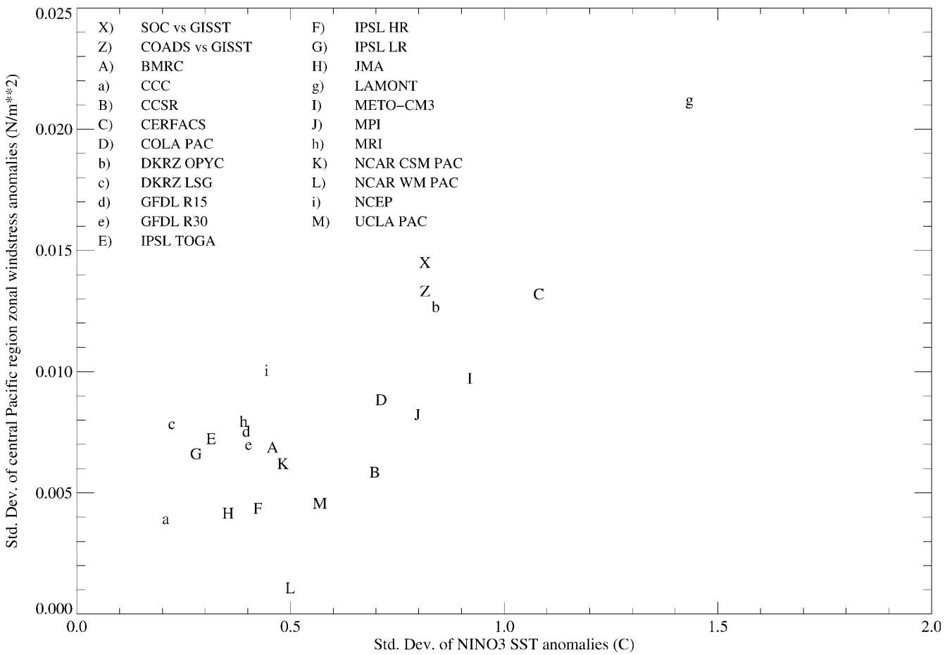
Fig. 5 Scatterplot of interannual standard deviations of SST (degrees C) in region Niño3 and zonal wind stress ( N\ m^{-2} ) in the central equatorial Pacific ( 5^{\circ}N-5^{\circ}S,165^{\circ}E-225^{\circ}E ). Lower case symbols indicate models with flux adjustment, while X and Z indicate observed values
