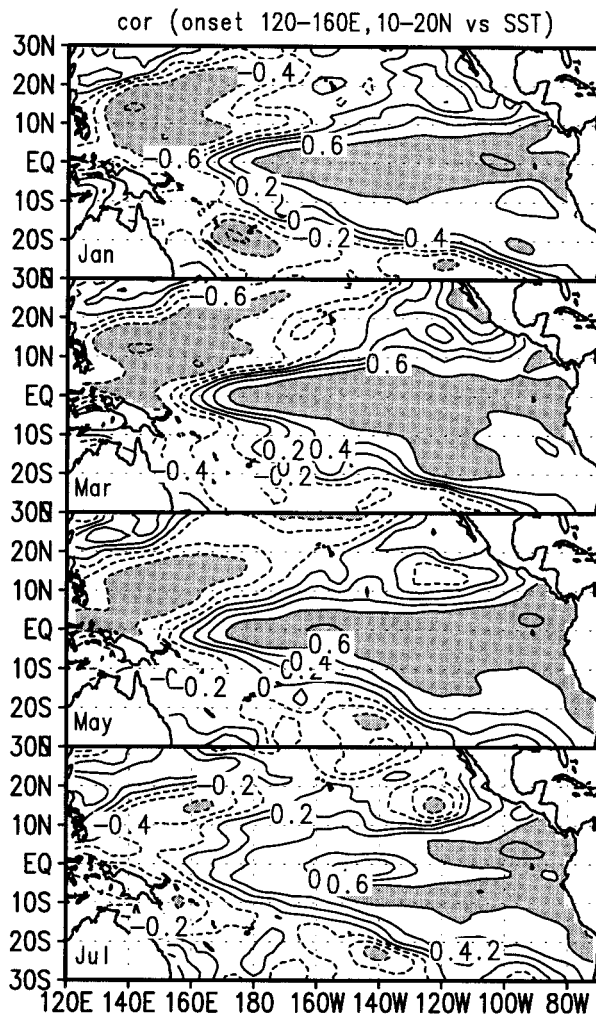
FIG. 5. Correlation maps of the onset anomaly averaged over the WNP ( 10^{\circ} – 20^{\circ} N, 120^{\circ} E– 160^{\circ} E) with SST anomalies in Jan, Mar, May, and Jul during 1980–95. Shaded regions are for correlation coefficients exceeding 0.6 that are significant over 95% confidence level according to an estimation of the decorrelation time (Livezey and Chen 1983).
