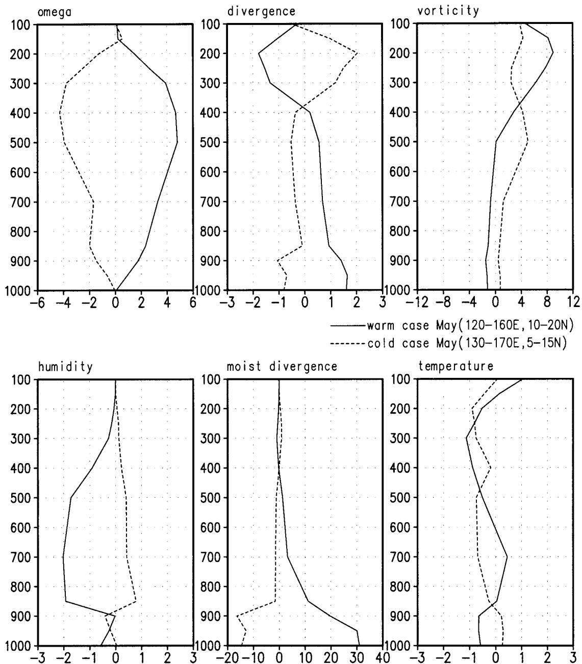
FIG. 11. The same as Fig. 6 except that the results are derived from numerical experiments for the model warm case over 10^{\circ} – 20^{\circ} N, 120^{\circ} – 160^{\circ} E (solid curves) and cold case over 5^{\circ} – 15^{\circ} N, 130^{\circ} – 170^{\circ} E (dashed curves). A slight different area was chosen for the cold case considering the southeastward shift of the upper-level divergent wind anomalies and the lower-level anomalous cyclone over the WNP.
