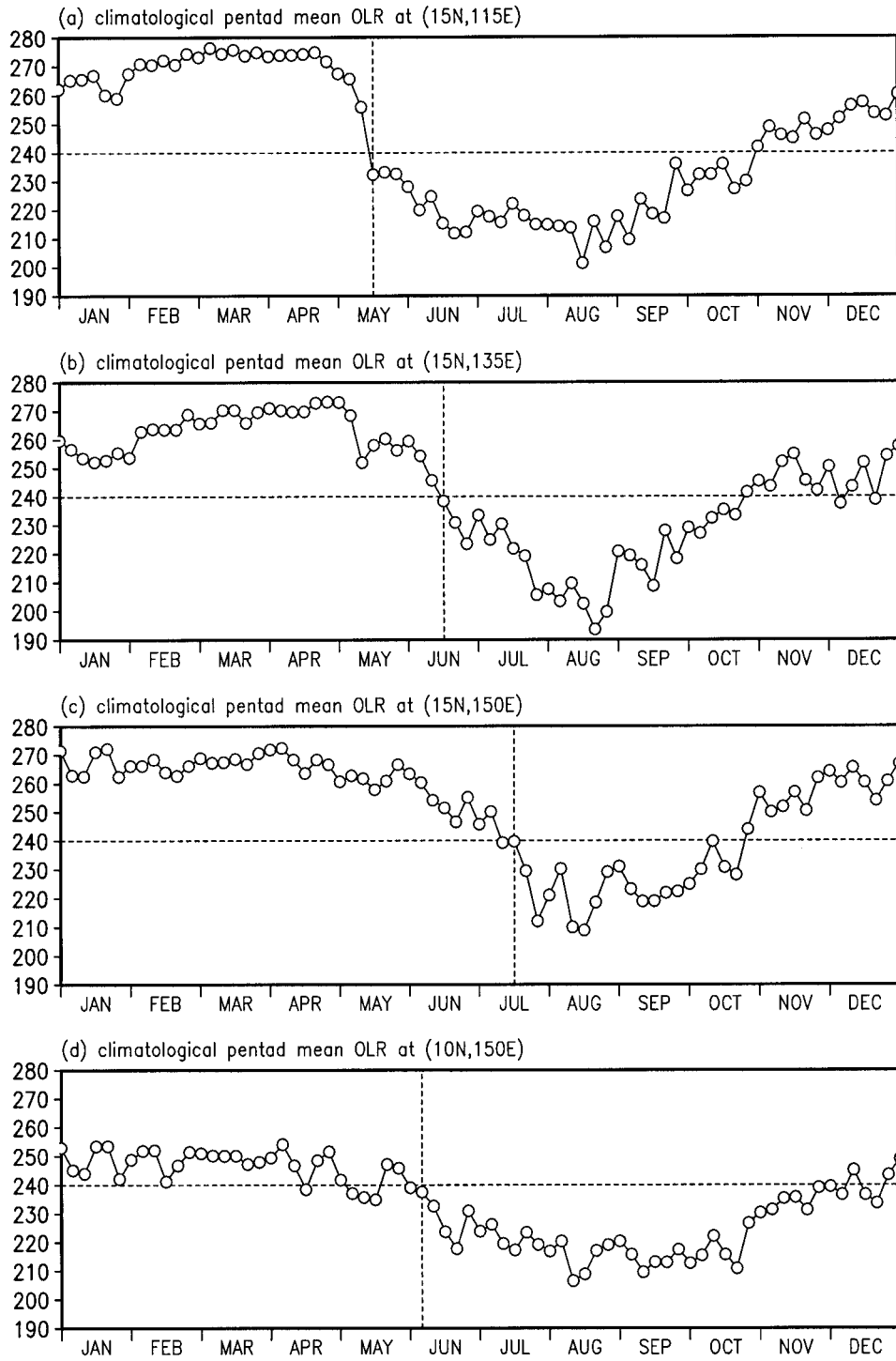
FIG. 1. Time series of climatological pentad mean OLR ( W m^{-2} ) at (a) 15^{\circ}N and 115^{\circ}E , (b) 15^{\circ}N and 135^{\circ}E , (c) 15^{\circ}N and 150^{\circ}E , (d) 10^{\circ}N and 150^{\circ}E . The dashed vertical lines indicate the onset dates.
