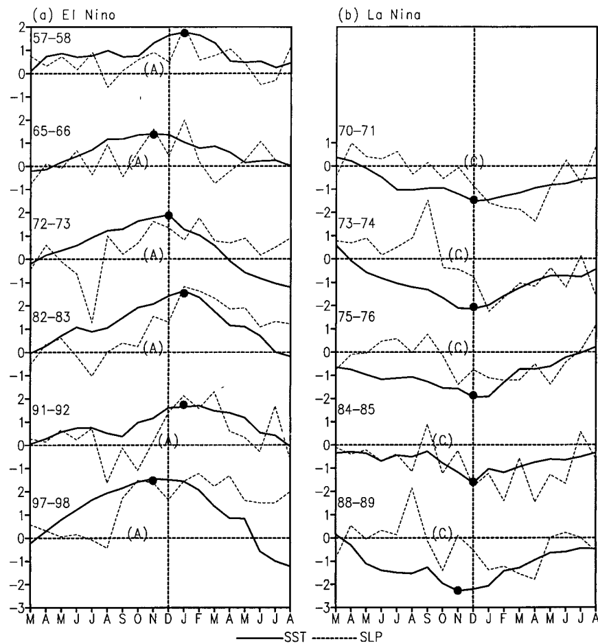
FIG. 9. Monthly mean SST anomalies ( ^{\circ}\text{C} ) at Niño-3.4 region (solid) and sea level pressure anomalies (hPa) over the Philippine Sea ( 10^{\circ} – 20^{\circ}\text{N} , 120^{\circ} – 150^{\circ}\text{E} ) (dashed) during the mature phases of (a) the six warmest and (b) the five coldest episodes shown in Fig. 1. Symbols (A) and (C) indicate the timing of the rapid establishment of the anomalous Philippine Sea anticyclone (cyclone). The black dots denote the times of the warm and cold peaks.
