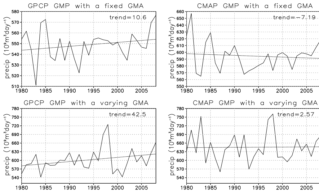
Figure 1. Time series of the global monsoon precipitation (GMP, unit: 10^9 \text{ m}^3 \text{ day}^{-1} ) calculated based on a (top) fixed and (bottom) varying global monsoon domain from the (left) GPCP and (right) CMAP datasets for the period of 1979–2008. The linear trend of each time series is presented by a dashed line, with a value of the linear trend [unit: 10^9 \text{ m}^3 \text{ day}^{-1} ( 29 \text{ yr}^{-1} )] shown in each panel.
