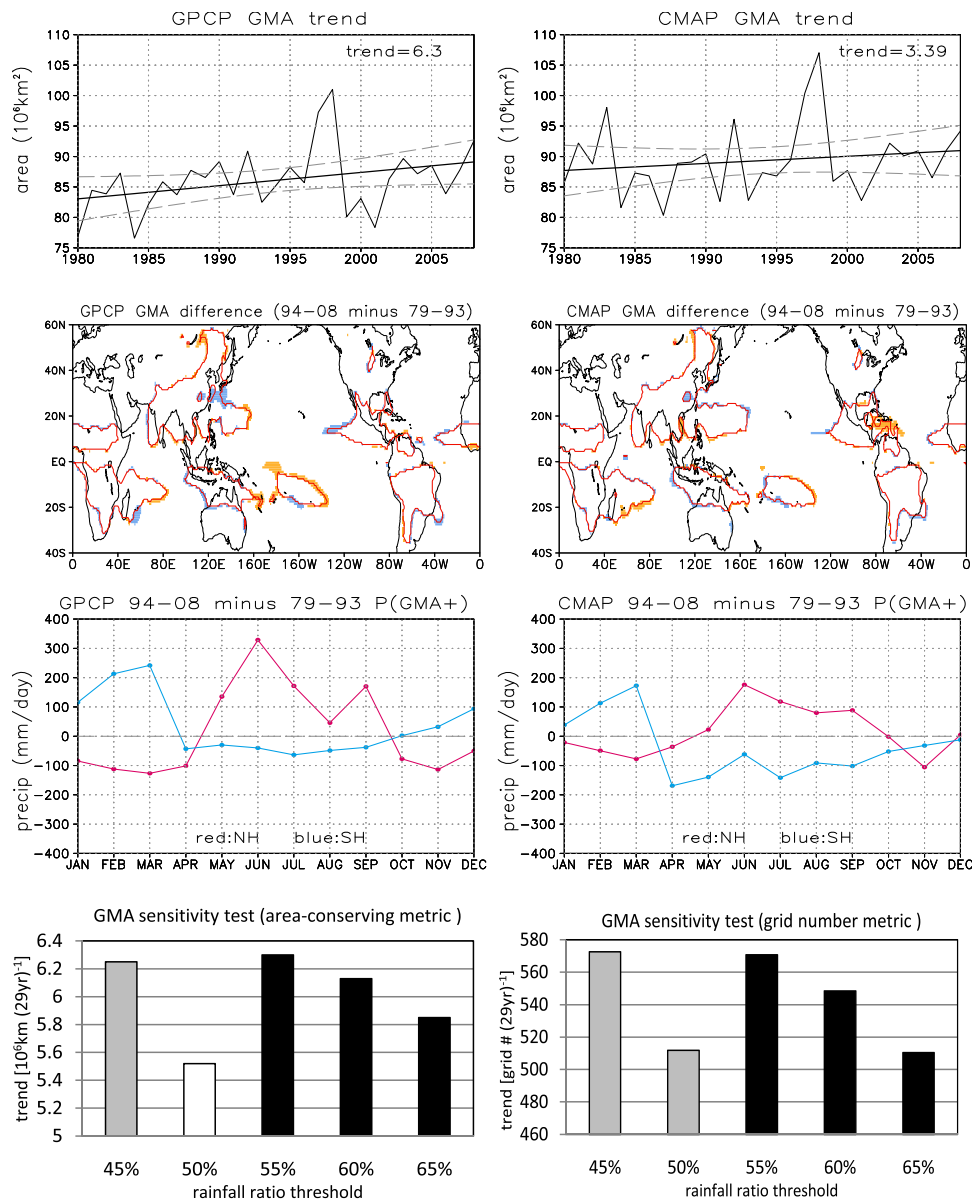
Figure 2. (top) Time series of the global monsoon area (GMA, unit: 10^6 \text{ km}^2 ) calculated based on the (left) GPCP and (right) CMAP datasets for the period of 1979–2008. The linear trend of each time series is presented by a thick black line, with a value of the linear trend [unit: 10^6 \text{ km}^2 (29 \text{ yr})^{-1} ] shown in each panel. Dashed lines indicate 95% confidence intervals for the GMA trends. (middle top) The difference of the GMA between 1994–2008 and 1979–1993. Blue (orange) shading indicates the positive (negative) GMA anomaly. Red contours denote the climatological GMA calculated based on averaged precipitation during 1979–2008. (middle bottom) The difference of seasonal precipitation distribution between 1994–2008 and 1979–1993 over expanding GMA regions in the Northern (red line) and Southern (blue line) hemisphere respectively. (bottom) GMA changes using different thresholds of summer-to-annual rainfall ratios in the GPCP. GMA calculations based on both the area-conserving [ 10^6 \text{ km}^2 (29 \text{ yr})^{-1} ] and unit grid metrics [ 1^\circ \times 1^\circ \text{ grid} \# (29 \text{ yr})^{-1} ] are shown in Figures 2 (bottom left) and 2 (bottom right), respectively. Trends exceeding 95% (90%) confidence level are indicated by black (gray) bars.
