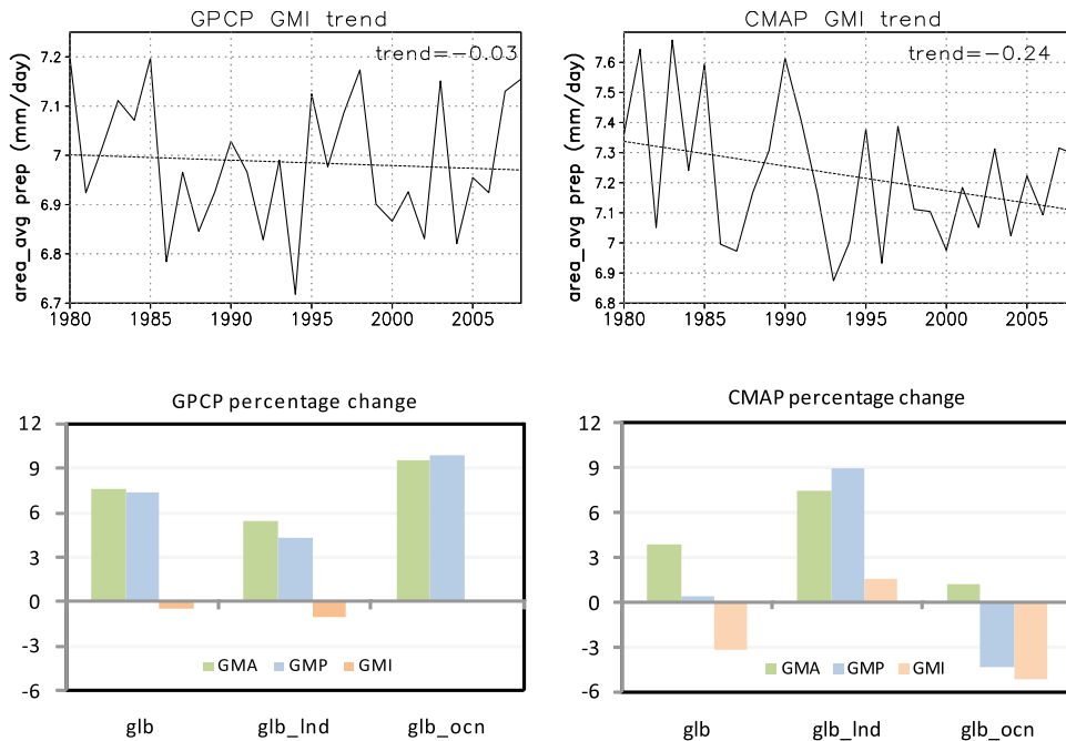
Figure 3. (top) Time series of the global monsoon intensity (GMI, unit: \text{mm day}^{-1} ) calculated based on the (left) GPCP and (right) CMAP datasets for the period of 1979–2008. The linear trend of each time series is presented by a dashed line, with a value of the linear trend [unit: \text{mm day}^{-1} ] shown in each panel. (bottom) Percentage changes (unit: %) of the GMA (green), GMP (blue) and GMI (orange) calculated from the (left) GPCP and (right) CMAP datasets in the global monsoon domain (denoted by “glb”), the global land monsoon region (“glb_lnd”), and the global oceanic monsoon region (“glb_ocn”).
