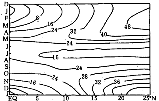
Fig. 9. As in Fig. 4 but for experiment A (unit: m/s).
