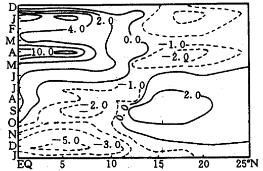
Fig. 17. As in Fig. 16 but for sensible heat flux ( W/m^2 ).
