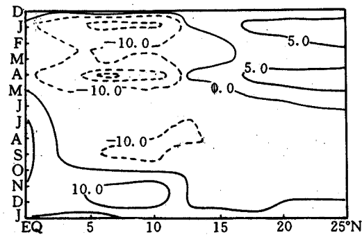
Fig. 16. As in Fig. 11 but for experiment B ( W/m^2 ).
