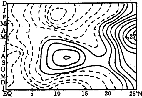
Fig. 2. The observation zonal wind at the underlying surface along 110°W (from paper by Murakami et al. 1992) (interval 1.0 m/s, dashed lines for easterly).
