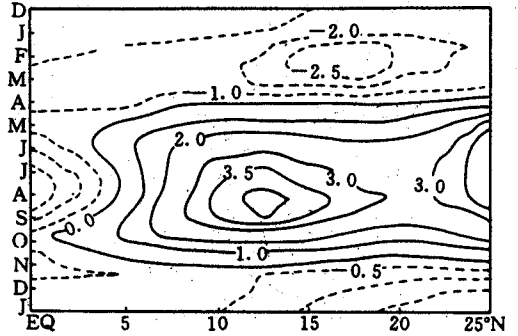
Fig. 5. As in Fig. 2 but for the control experiment (unit: m/s).
