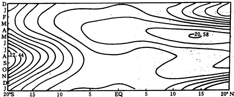
Fig. 1. The latitude-time distribution of SST along 110^{\circ}\text{W} (interval 0.5^{\circ}\text{C} ) (from paper by Murakami et al. 1992).
