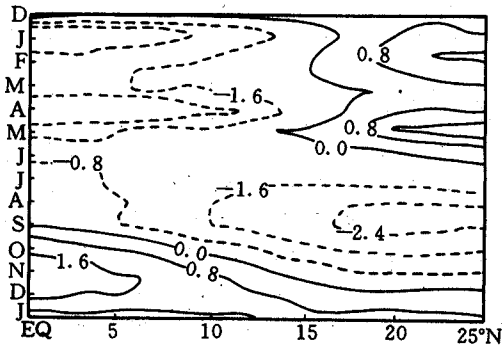
Fig. 18. As in Fig. 16 but for atmospheric temperature at 900 hPa ( ^{\circ}\text{C} ).
