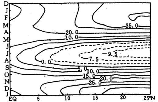
Fig. 15. As in Fig. 9 but for experiment B (m/s).
