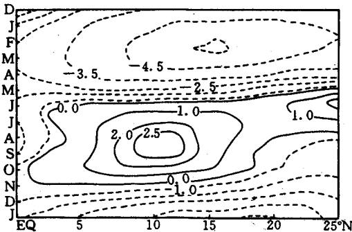
Fig. 8. As in Fig. 2 but for experiment A (m/s).
