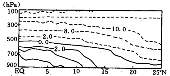
Fig. 13. The latitude-altitude distribution of mean temperature difference between the sensitivity experiment A and the control experiment in May ( ^{\circ}\text{C} ).
