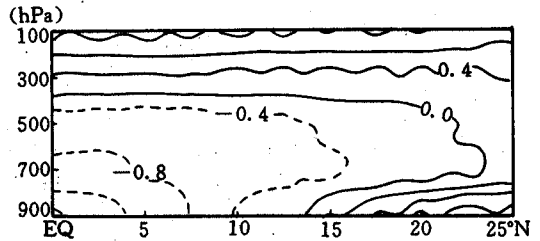
Fig. 19. As in Fig. 13 but for experiment B ( ^{\circ}\text{C} ).
