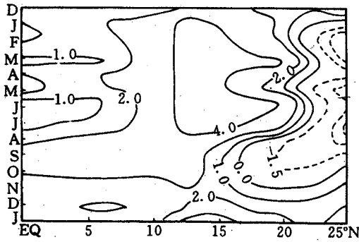
Fig. 12. As in Fig. 10 but for the temperature difference at 900 hPa ( ^{\circ}\text{C} ).
