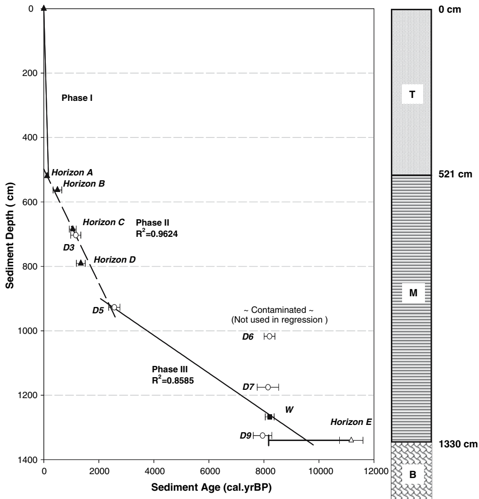
Fig. 3 Complete chronology of Ordy Pond sediment. Dates of horizons A, B, C, and D ( closed triangles ) are from Athens et al. (1999, 2002) and that of horizon E ( open triangle ) is from Tribble et al. (1999). Dates of n -alkanes from horizon D3, D5, D6, D7, and D9 ( open circles ) were determined by CSRA and that of wood fragments from horizon W ( closed square ) was from AMS. The two types of error bars on the snail date represent an analytical and statistical error, and an arbitrary error of 3,000 cal.yrBP due to limestone-effect. Three distinct
