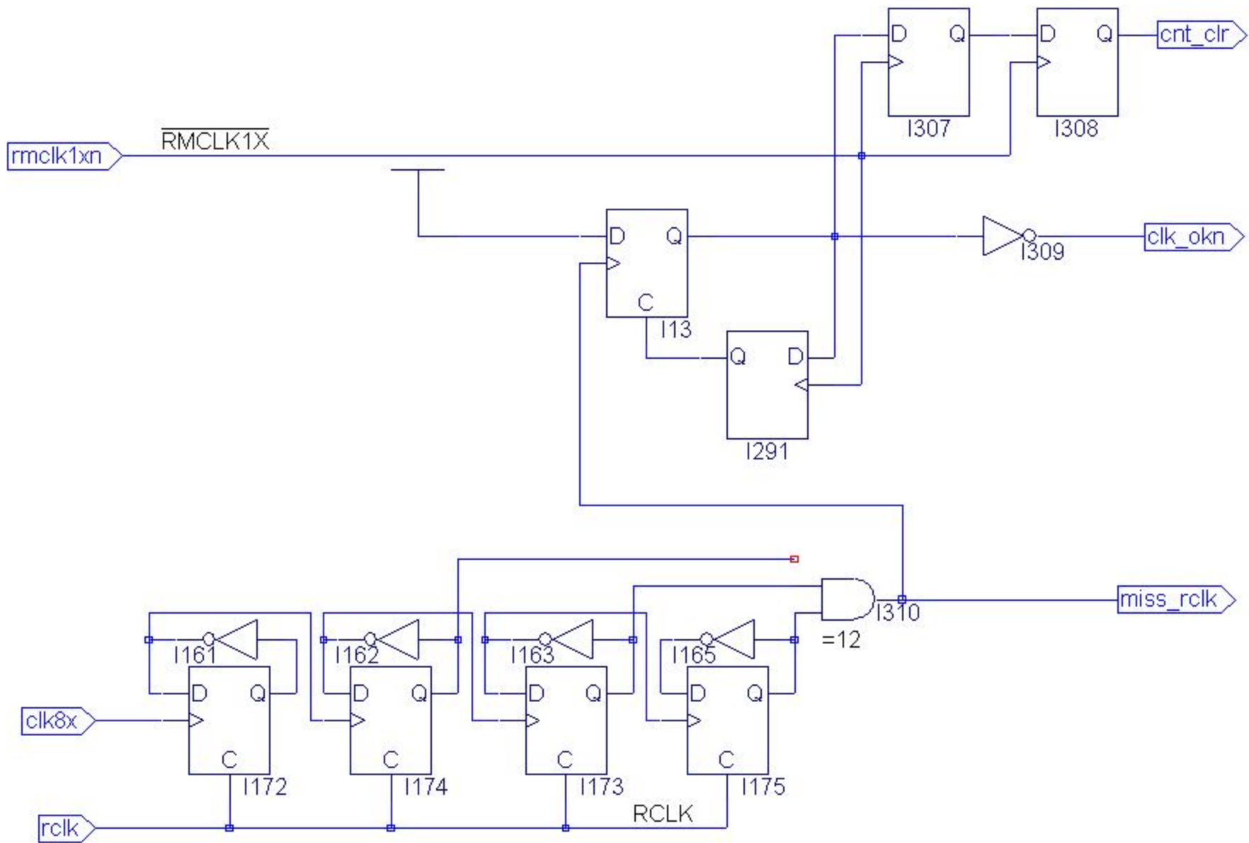
Missing RCLK - Manchester Violation
